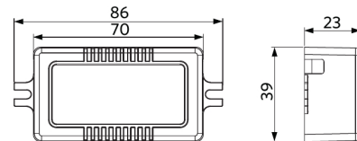
LEDspotRA-Ava-E2 Driver
