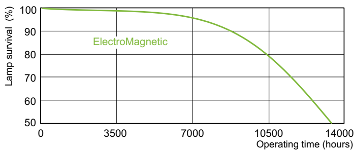
Life Expectancy Diagram - MASTER PL-S 11W/840/2P 1CT/5X10BOX
