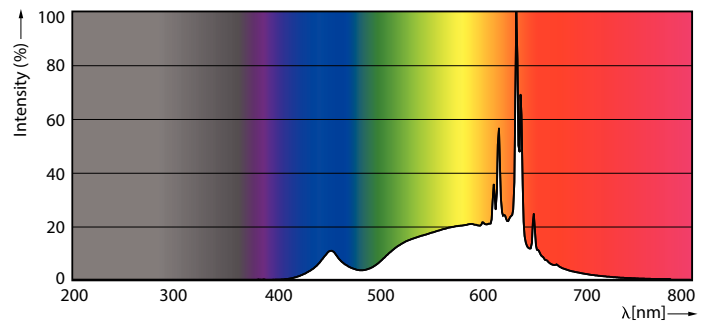
Spectral Power Distribution Colour - CorePro LEDspot 3-35W GU10 827 36D DIM
