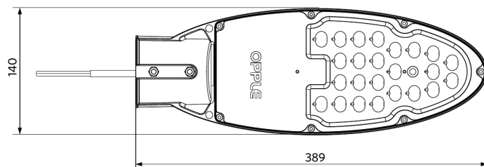
LEDStreet-SE-ExtensionCable
