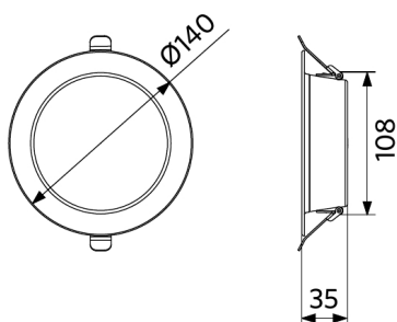
LEDDownlightCo-E Rd125
