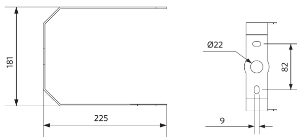
LEDHighbay-P5 Bracket-D420
